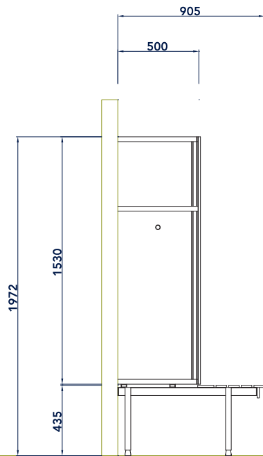
SEATING LOCKER COMBO SECTION
