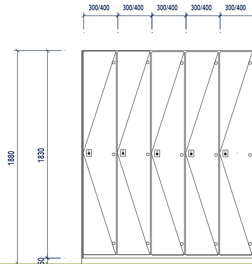
1 TIER FRONT ELEVATION
